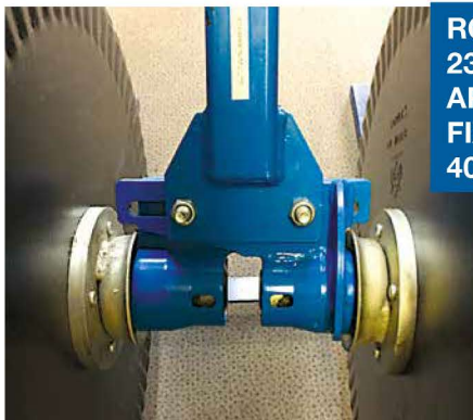
HEAVY DUTY ADJUSTABLE VERSION, SHOWING TAPERED ROLLER BEARING ASSEMBLIES
